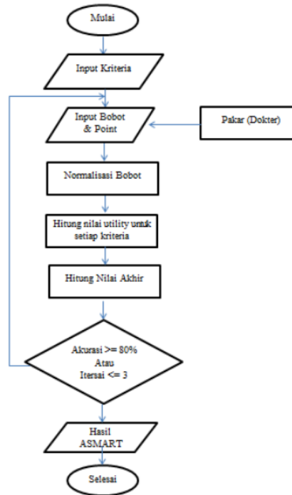
Gambar 1. Flowchart ASmart
