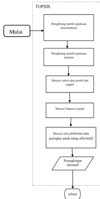
Gambar 9. Flowchart algoritma TOPSIS
